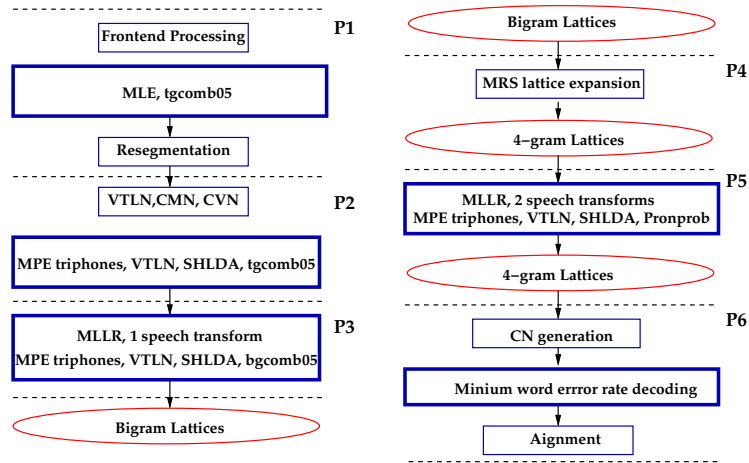
Fig. 4. Processing stages of AMI system for 2005 NIST evaluations. The figure is reprinted from [5] with permission of the author.
