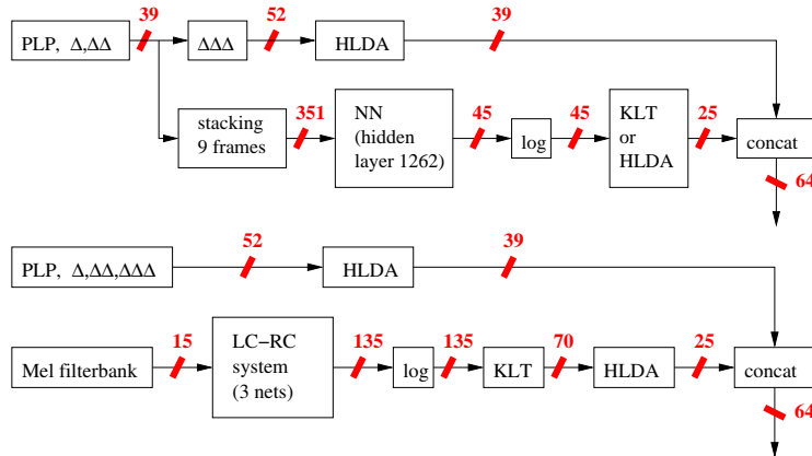
Fig. 3. Configuration of the system with PLP- (upper panel) LCRC-posteriors (lower panel).
