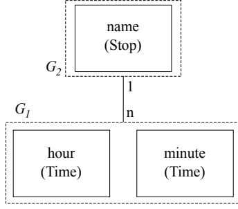
Figure 4: A domain graph model corresponding to the domain model shown in Figure 1 that represents the property groups and the relationships among them.
