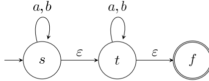
Figure 4.2: One-turn all-move self-regulating finite automaton M .
