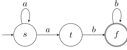
Figure 4.1: One-turn first-move self-regulating finite automaton M .
