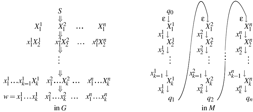
Figure 4.3: A derivation of w in G and the corresponding acceptance of w in M .
