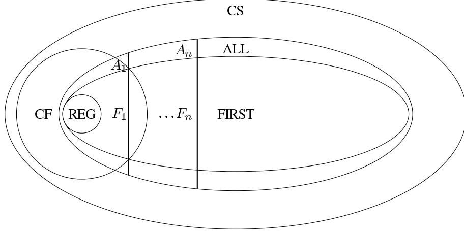
Figure 4.4: The hierarchy of languages. Here, F_n stands for FIRST_n , and A_n for ALL_n .
