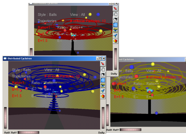
Fig. 89: Distributed cyclotron
