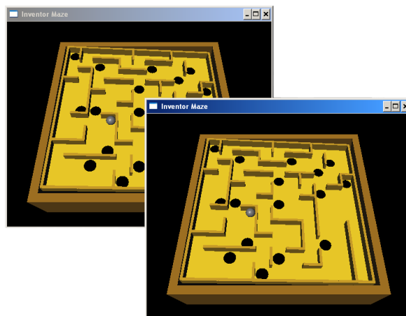
Fig. 85: Collaborative Maze
