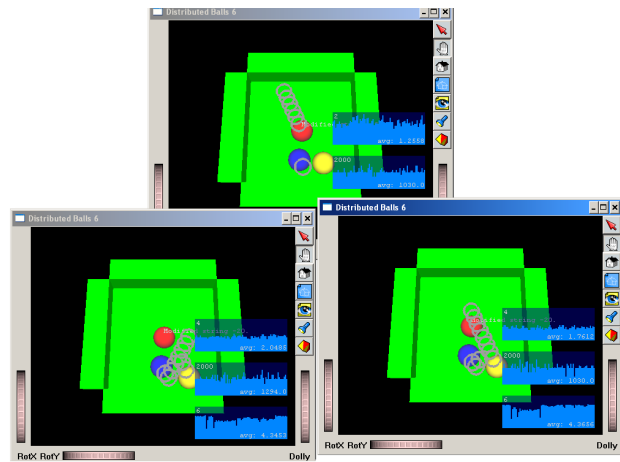
Fig. 88: Distributed billiard
