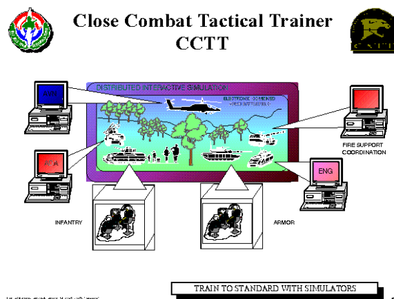
Fig. 6: DIS simulation
