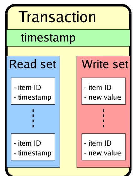
Fig. 60: Transaction structure
