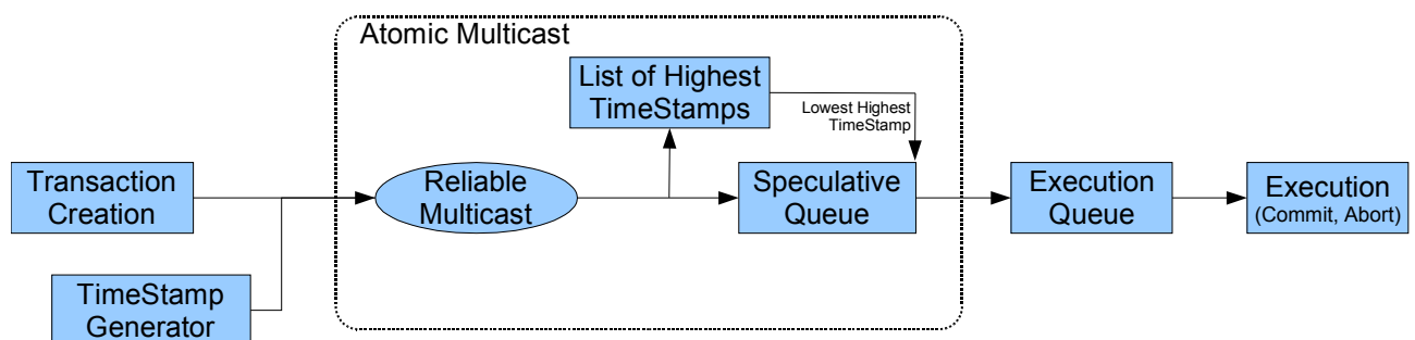
Fig. 61: Transaction processing
