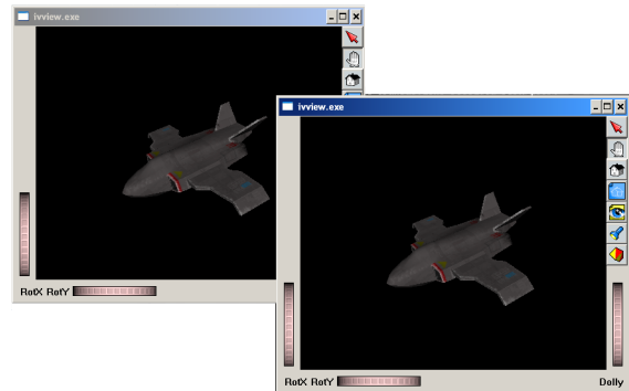
Fig. 84: Collaborative viewer
