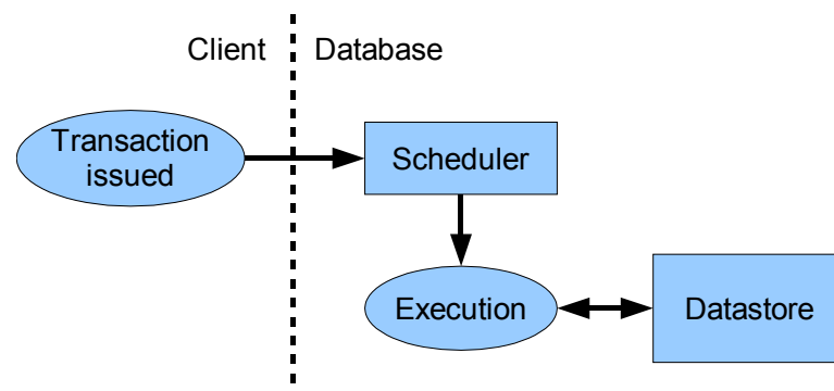
Fig. 35: Transaction processing
