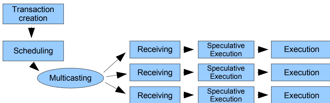
Fig. 63: Transaction execution
