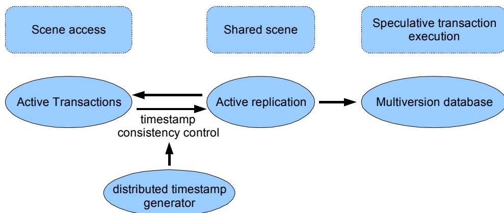
Fig. 56: Main concepts of Active transactions
