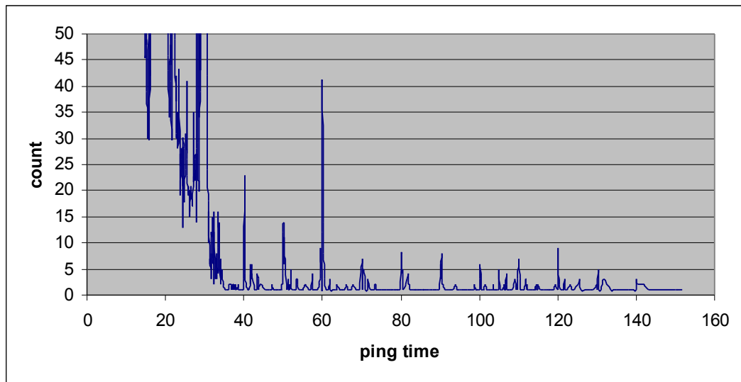
Fig. 108: Detailed round trip time of two computers on high-speed LAN
