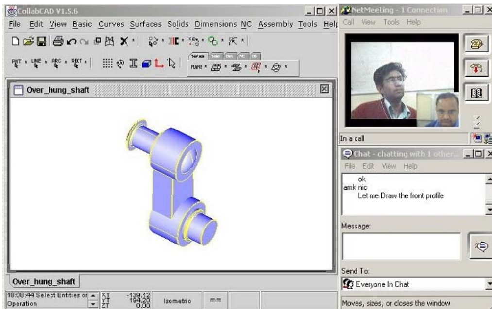
Fig. 8: CollabCAD
