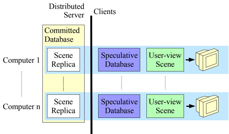
Fig. 67: Database model
