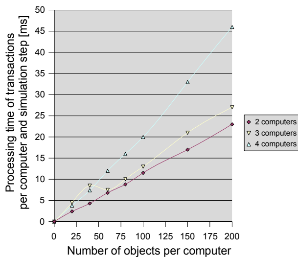
Fig. 100: Processing time of transactions with optimizations per simulation step
