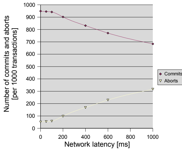
Fig. 104: Number of commits and aborts per 1000 executed transactions
