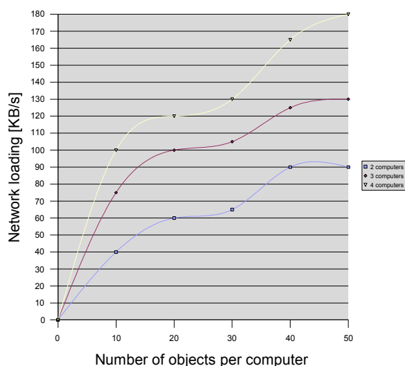
Fig. 90: Distributed cyclotron network loading (adaptive simulation step)
