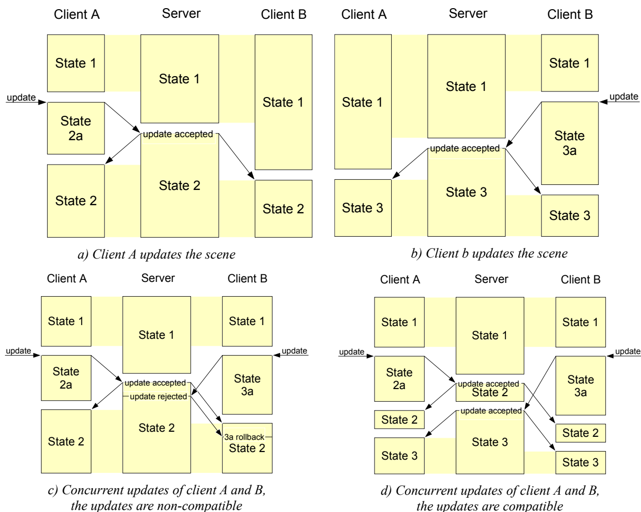
Fig. 40: Update concurrency
