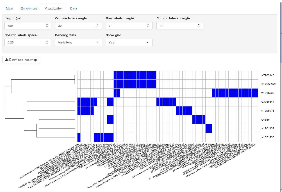
Figure 5-12. Visualization tab.
