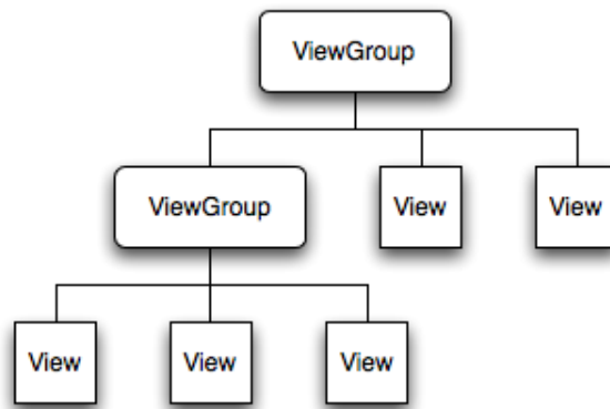
Obr. 4.3: ViewGroups
