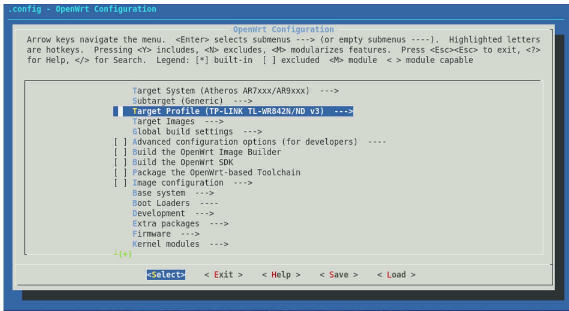
Figure 4.1: Menuconfig
