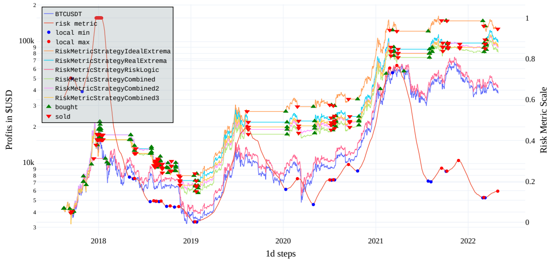
Figure 7.12: Showcase of evaluation strategies for the same risk metric.
