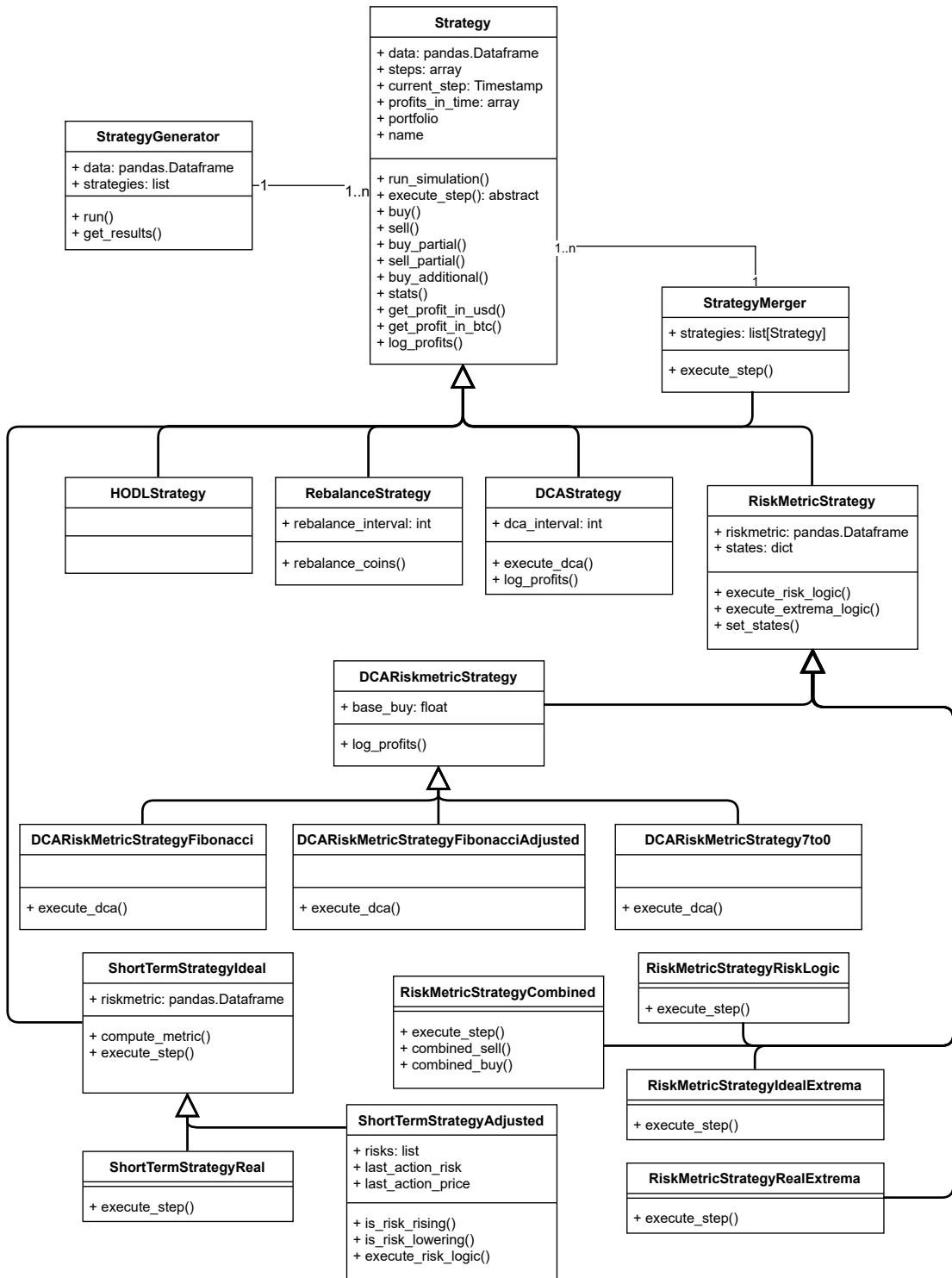
Figure 6.2: Class diagram of strategies of the backtester.
