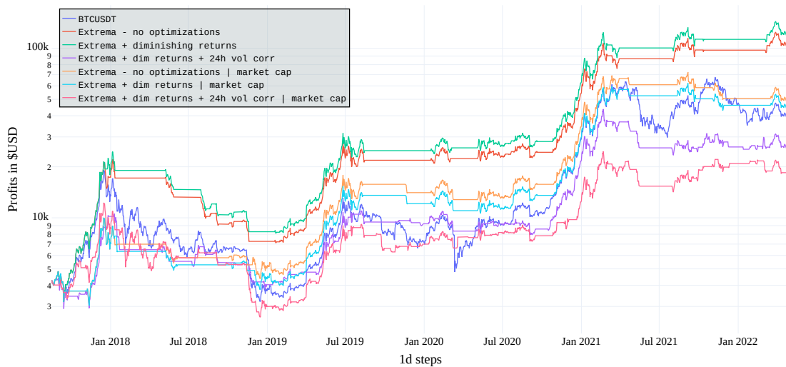
Figure 7.15: Comparison of risk optimizations used with the local extrema evaluation strategy. Dates: July 2017–May 2022.
