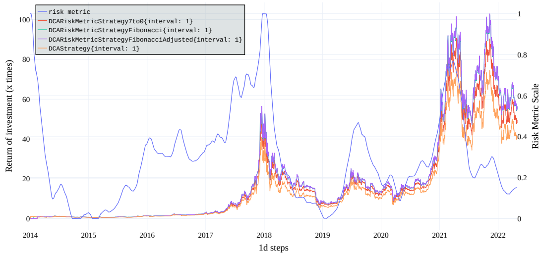
Figure 7.13: Showcase of evaluation strategies for the DCA strategy.
