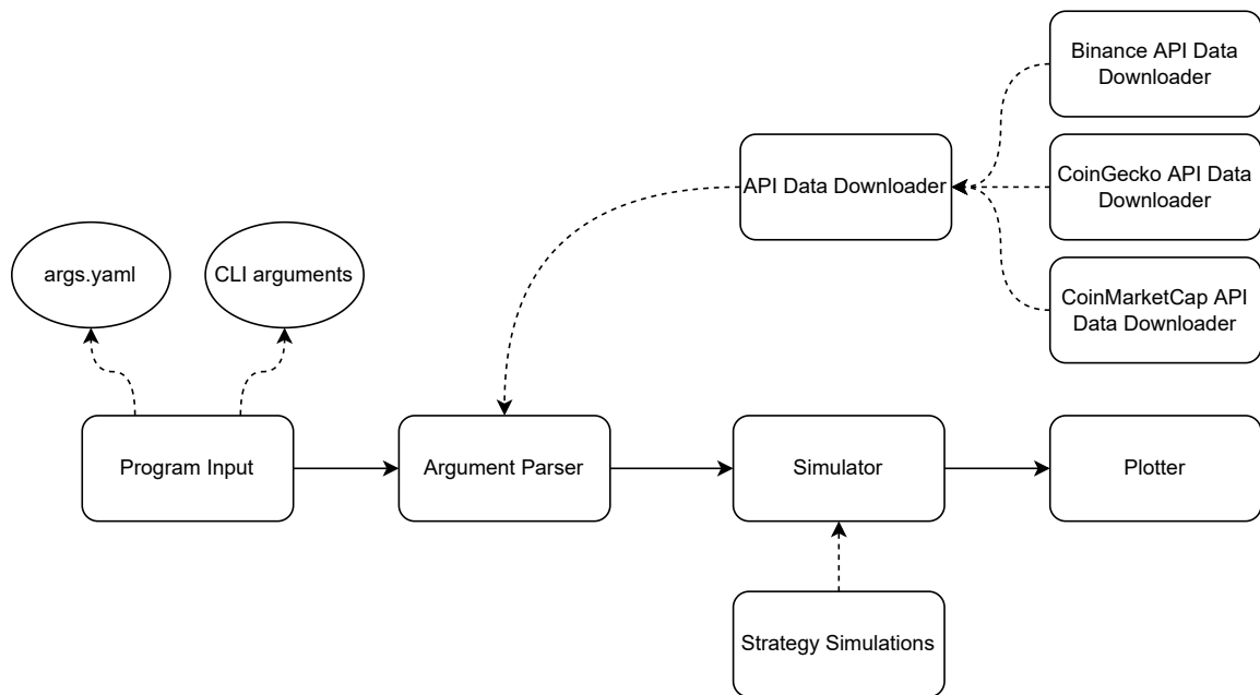
Figure 6.1: General design structure of the backtester.
