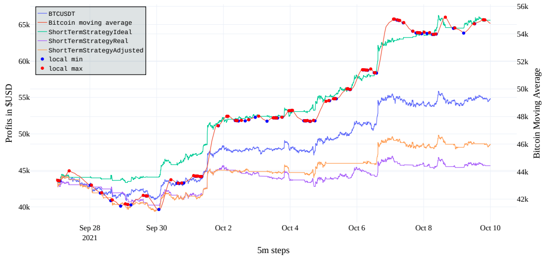
Figure 7.23: 27th Sep–10th Oct 2021 rising trend that registered rise from $43000 to $55000.
