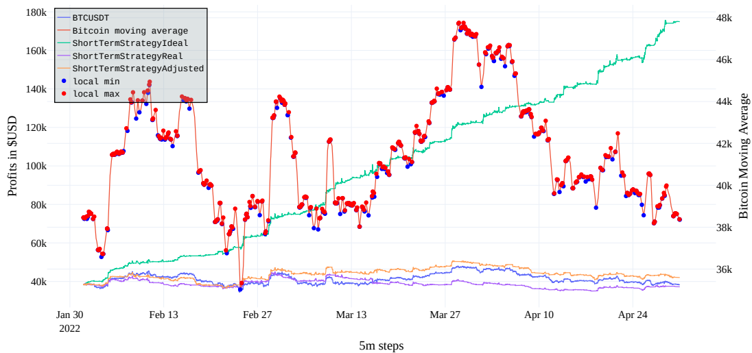
Figure 7.26: 1st Feb–30th Apr 2022 long date range.
