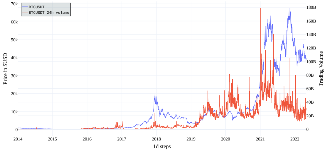
Figure 7.7: Linear graph comparison between Bitcoin price and its daily volume traded in $USD.
