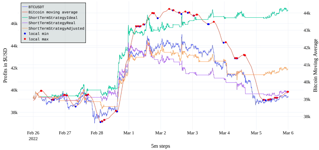
Figure 7.25: 26th Feb–6th Mar 2022 changing trend.
