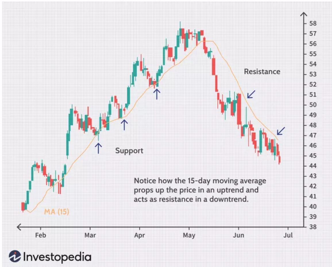
Figure 7.22: Expected support and resistance levels computed by a moving average. Attribution: Investopedia [43].
