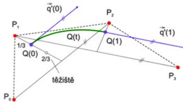
Obr. 4.4: Coonsova kubika
